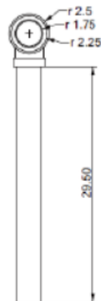
TOP VIEW
